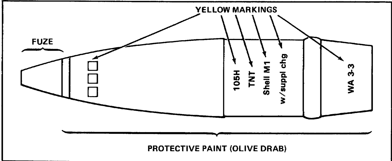
Figure 4. HE Projectile.
